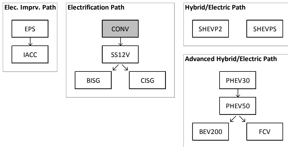
Figure-II-15 - Electrification Technology Path
