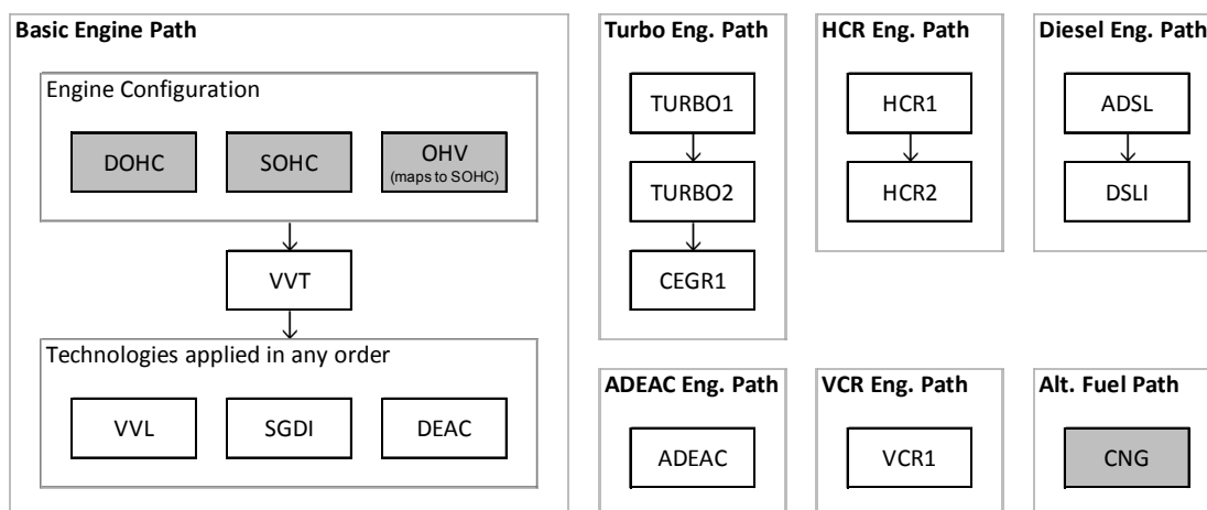
Figure-II-13 - Engine Paths
