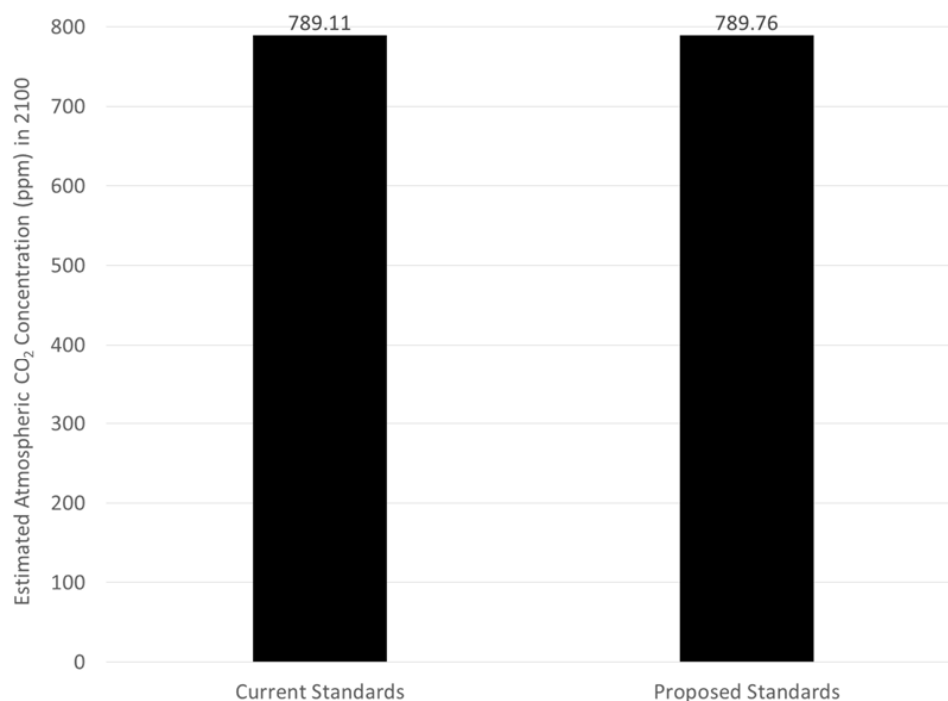
Figure I-4 - Estimated Atmospheric CO 2 Concentration in 2100
